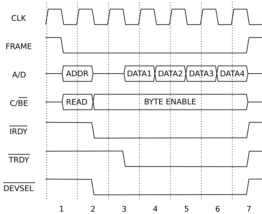
Figure 1-7. PCI Bus Read Cycle
