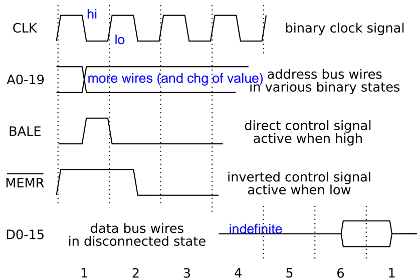
Figure 1-4. Timing Diagram Example
