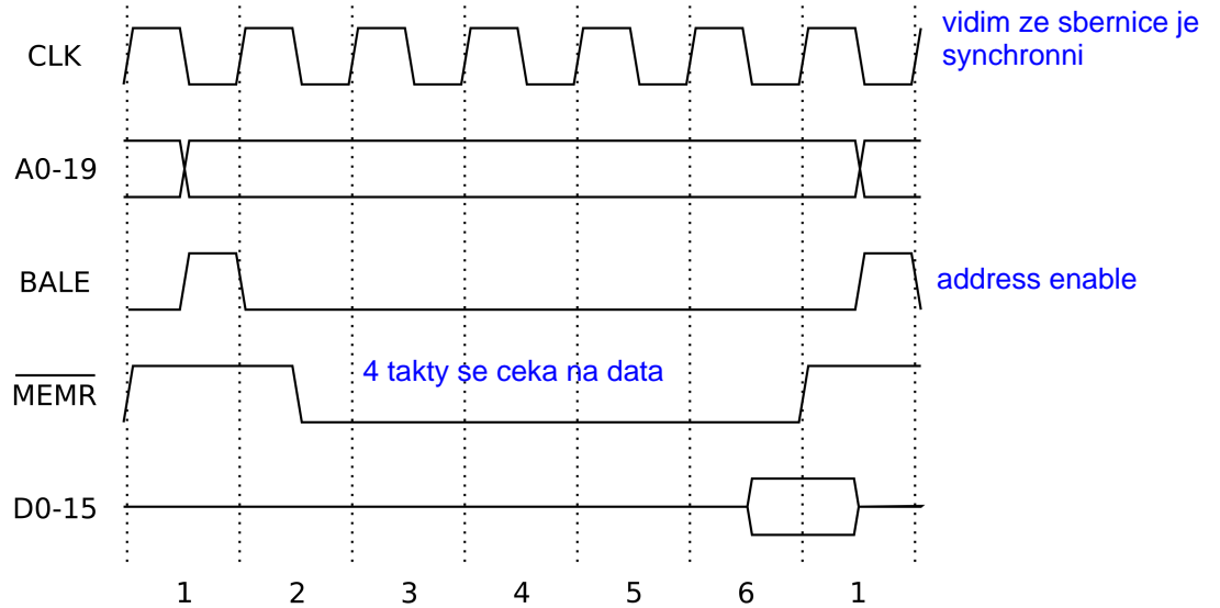
Figure 1-5. ISA Bus Read Cycle
