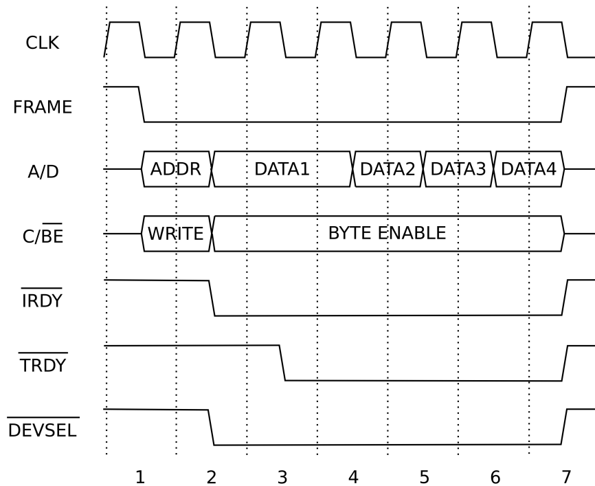
Figure 1-8. PCI Bus Write Cycle
