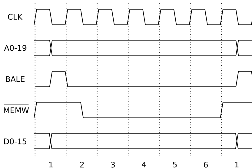
Figure 1-6. ISA Bus Write Cycle
