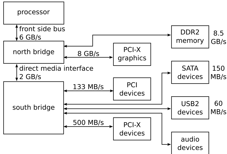
Figure 1-9. Multiple Busses Example
