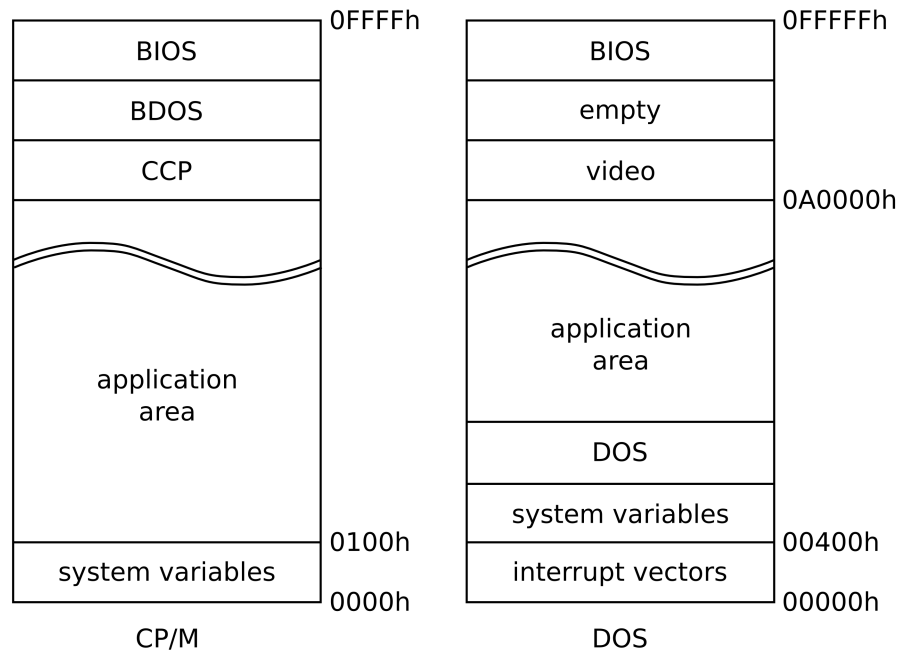
Figure 1-10. Simple Monolithic Operating Systems Example
