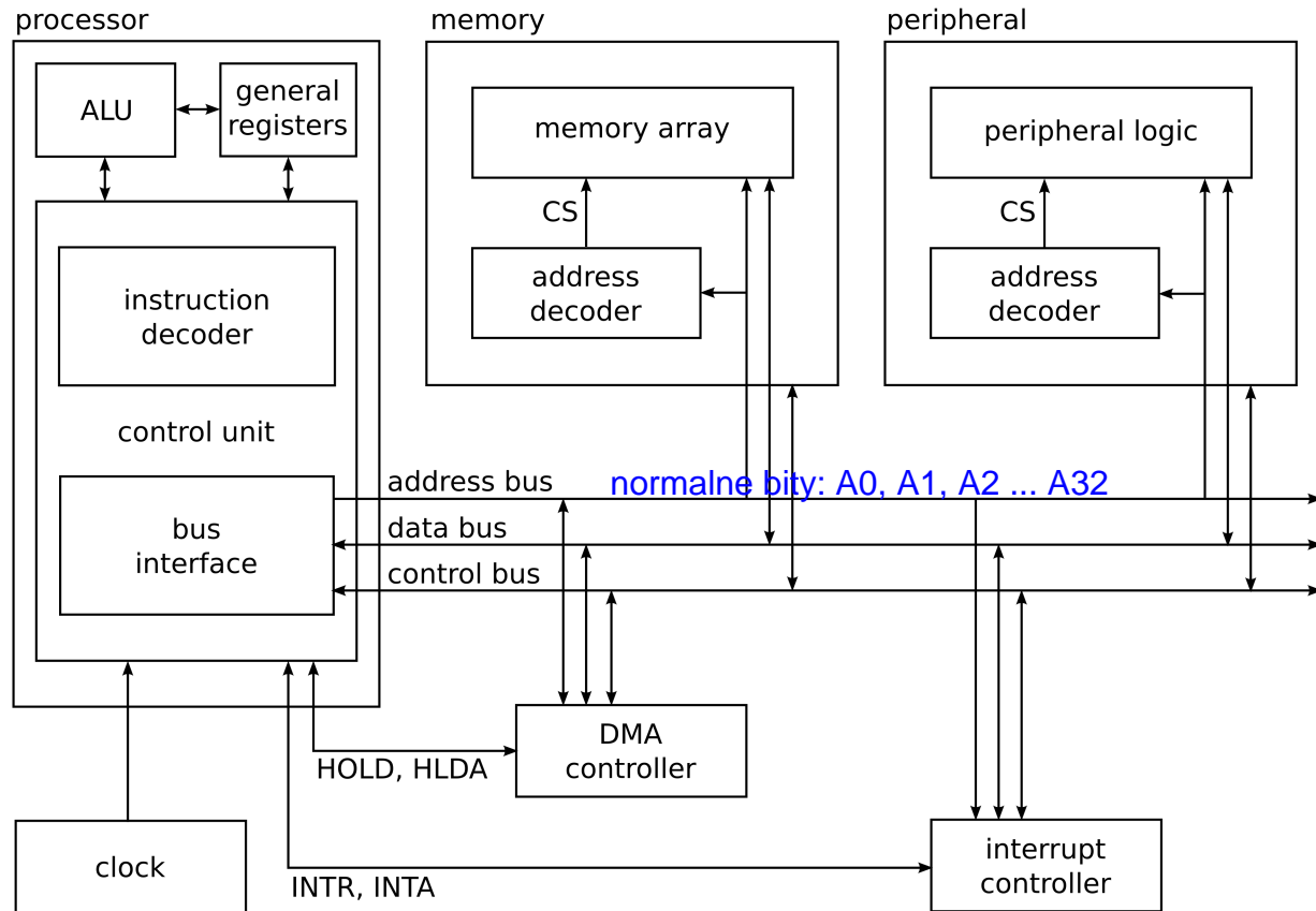
Figure 1-3. Basic Computer Architecture Example
